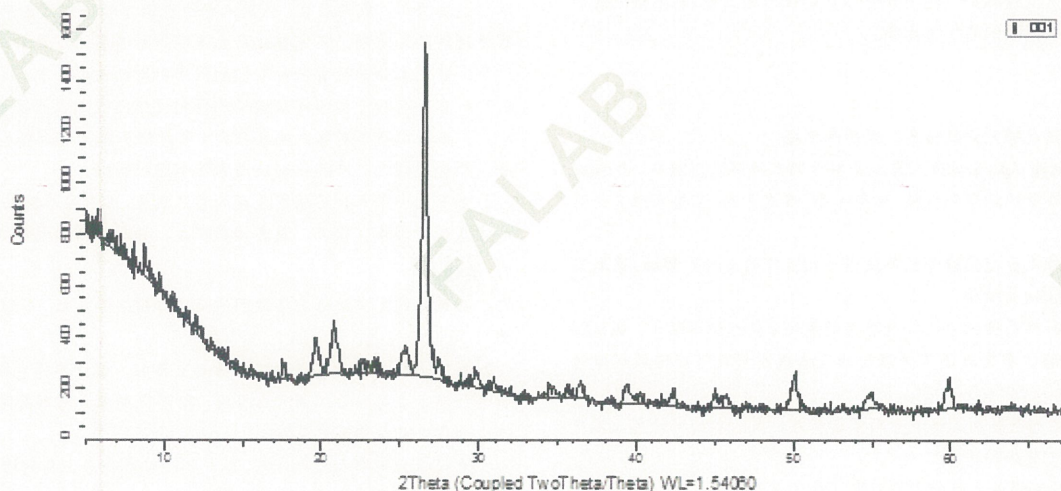
XRD spectrum
